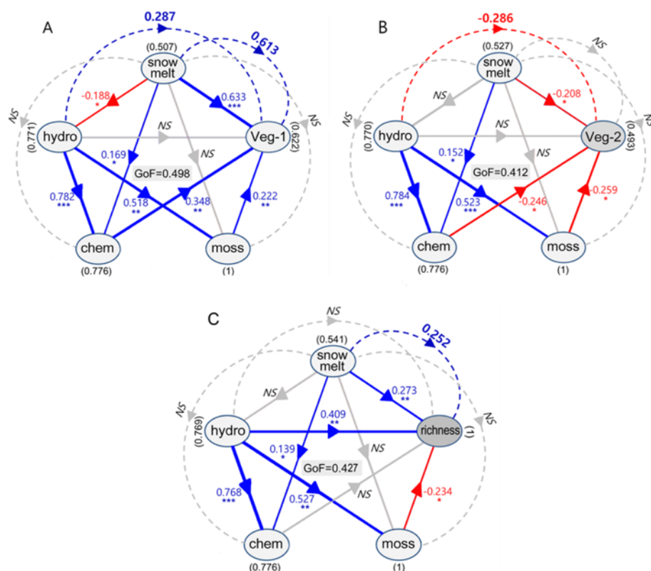
Fig. 4. Inner models in the partial least squares path model of effects of environmental parameters on Arctic plant abundance and distribution, showing path coefficients (numbers near the arrows) and average variance-extracted values (in parentheses). Blue arrows indicate positive relationships; red arrows indicate negative relationships. Straight lines indicate direct effects; dotted lines indicate total effects (=direct effects + indirect effects). The significance of each direct effect is estimated based on the regression equation between latent variables (NS, non-significant; * p < 0.1 ; ** p < 0.01 ; *** p < 0.001 ). The significance of each total effect is estimated based on the simulation-bootstrapped 95% confidence interval.
